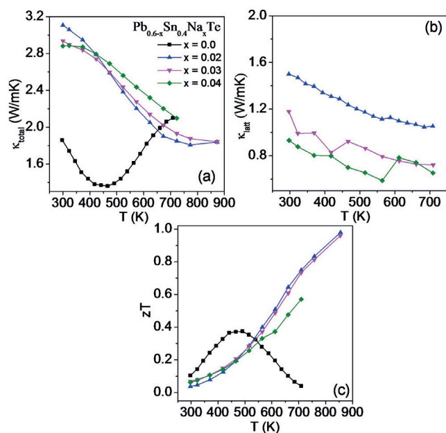
Figure 4. Temperature-dependent a) total thermal conductivity ( \kappa_{\text{total}} ), b) lattice thermal conductivity ( \kappa_{\text{latt}} ), and c) thermoelectric figure of merit ( zT ) of \text{Pb}_{0.6-x}\text{Sn}_{0.4}\text{Na}_x\text{Te} ( x=0-0.04 ) samples.
